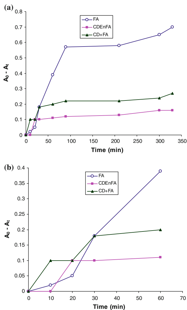
Fig. 8 Difference in absorbance versus length of time of irradiation of a 330 min and b 60 min for aqueous solution samples
