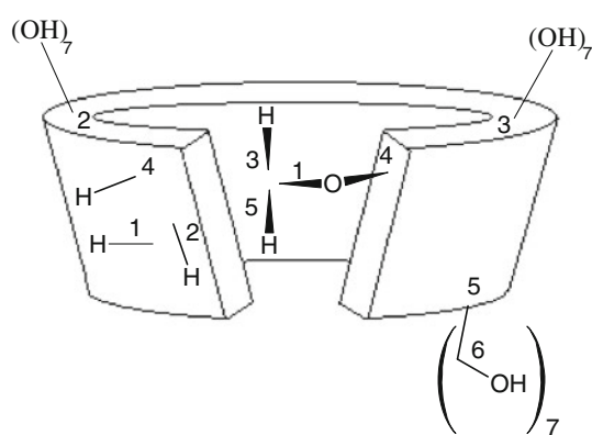
Fig. 2 Truncated-cone representation of \beta -cyclodextrin
