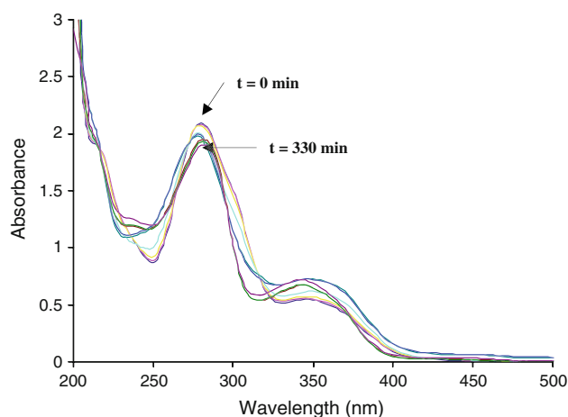
Fig. 7 Electronic absorption spectrum of an aqueous solution of a physical mixture of folic acid and \beta -cyclodextrin both at 1.68 \times 10^{-4}\text{ mol dm}^{-3} irradiated over 330 min
