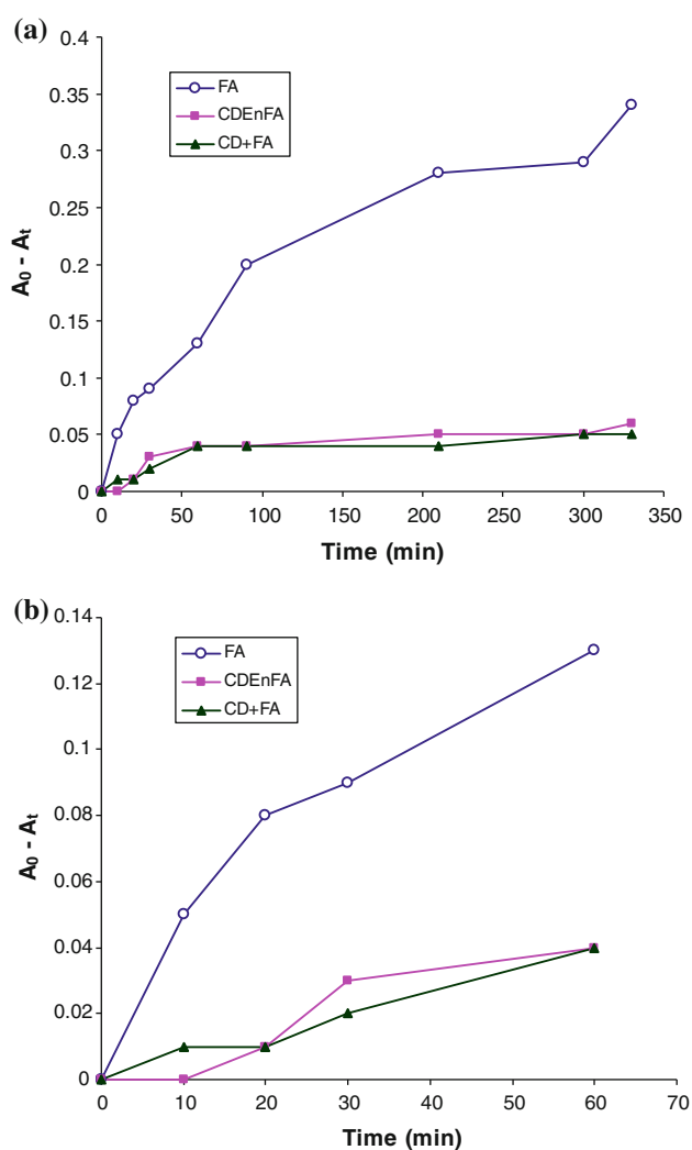
Fig. 9 Difference in absorbance versus length of time of irradiation of a 330 min and b 60 min for solid state samples of FA, CDEnFA and a physical mixture of both
