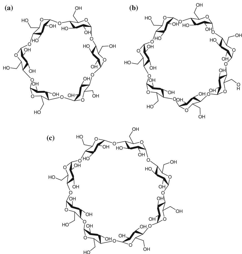
Fig. 1 Structure of a \alpha -cyclodextrin, b \beta -cyclodextrin and c \gamma -cyclodextrin
