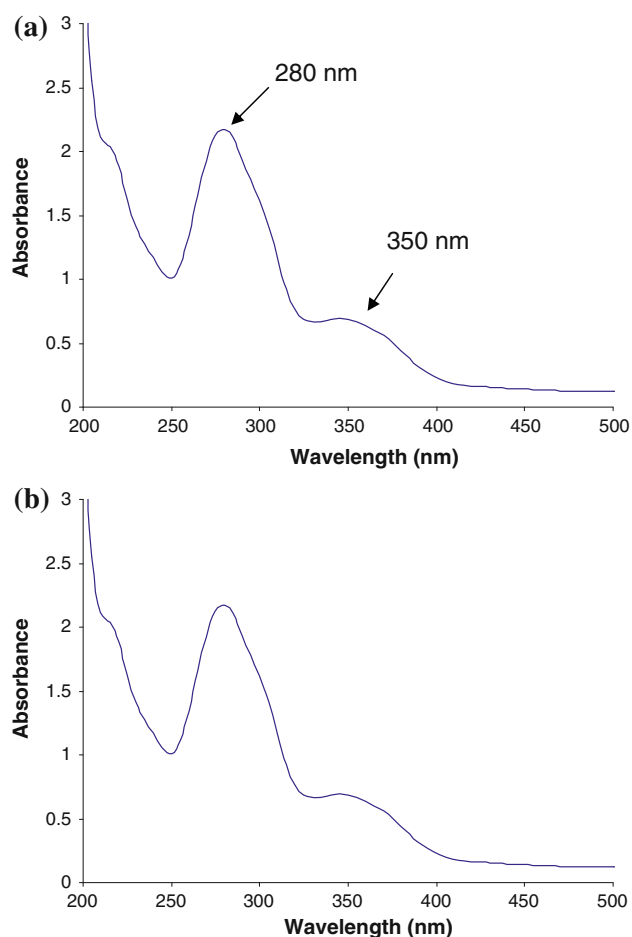
Fig. 5 Electronic absorption spectra of aqueous solutions of a folic acid and b CDEnFA both at 1.68 \times 10^{-5} \text{ mol dm}^{-3}
