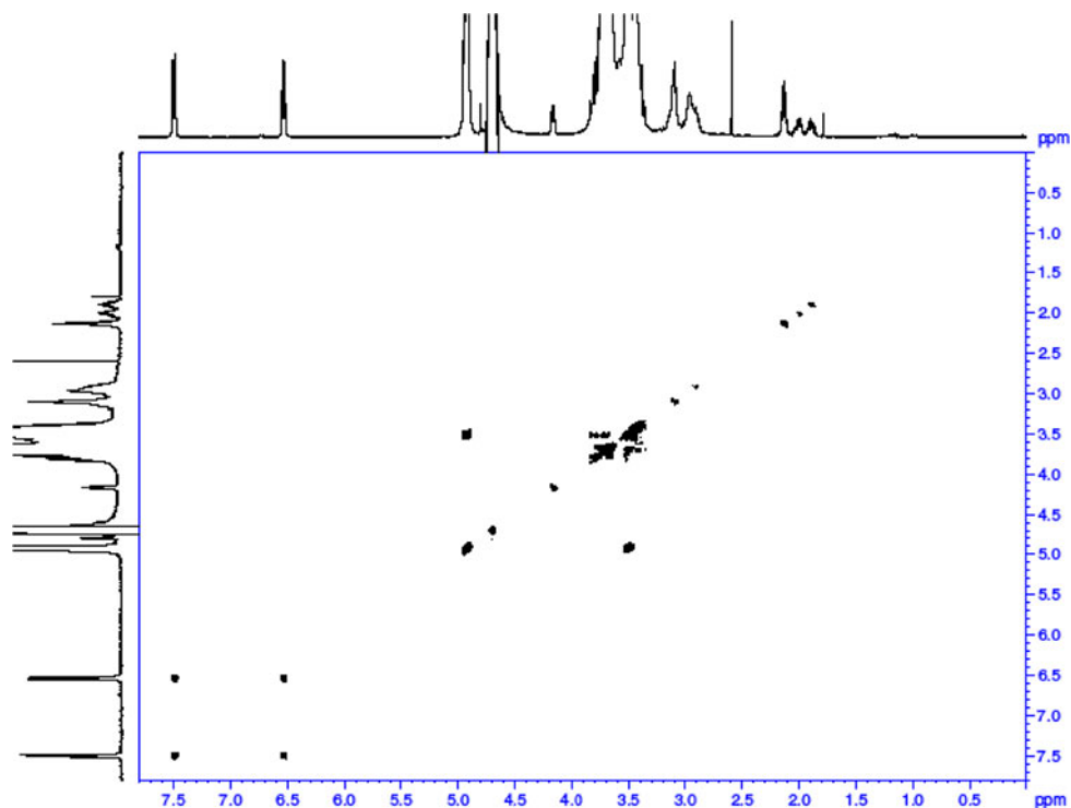
Fig. 4 COSY NMR of CDEnFA in D_2O at 30 °C
