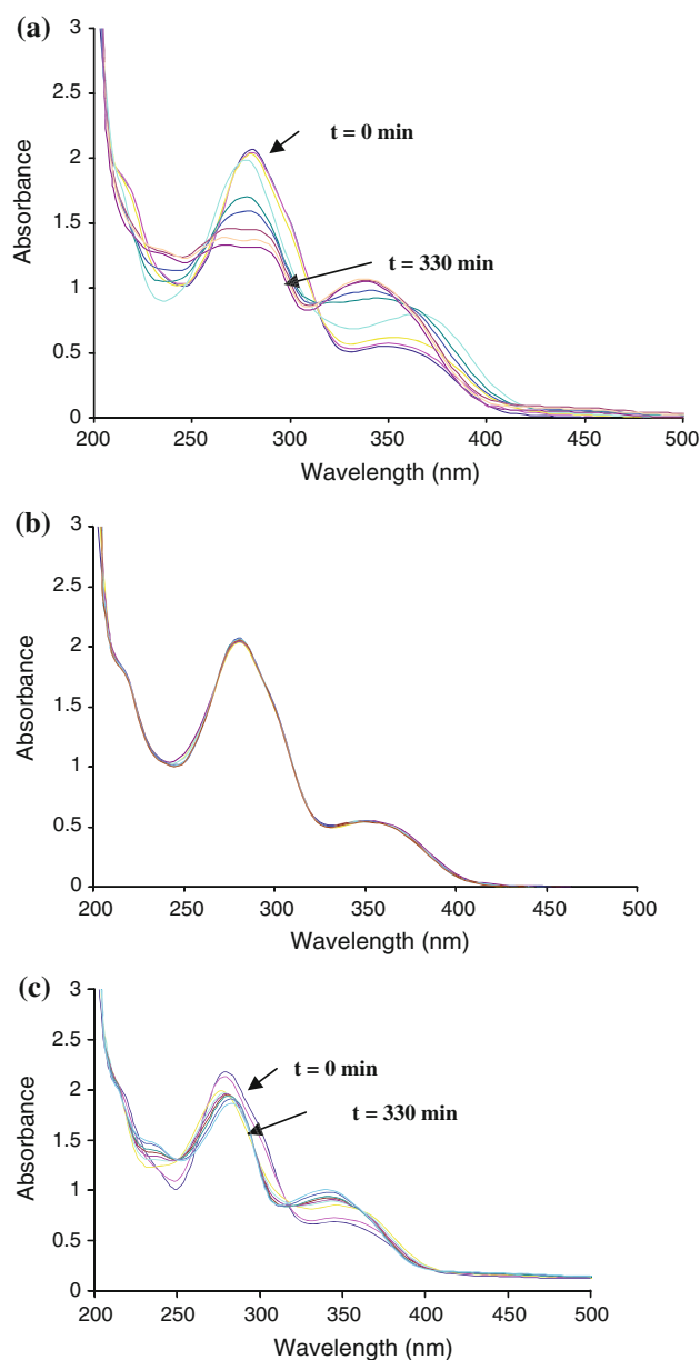
Fig. 6 Electronic absorption spectra of aqueous solutions of a folic acid irradiated over 330 min, b non-irradiated folic acid and c CDEnFA irradiated over 330 min (all at 1.68 \times 10^{-4} \text{ mol dm}^{-3} )
