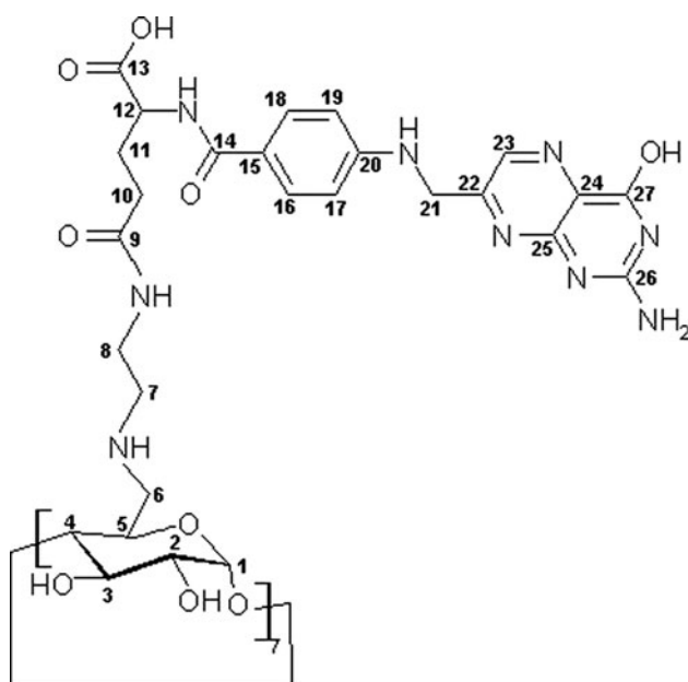
Fig. 3 Proposed structure of 6-deoxy-6-[(1-(2-amino)ethylamino)folate]- \beta -cyclodextrin (CDEnFA)
